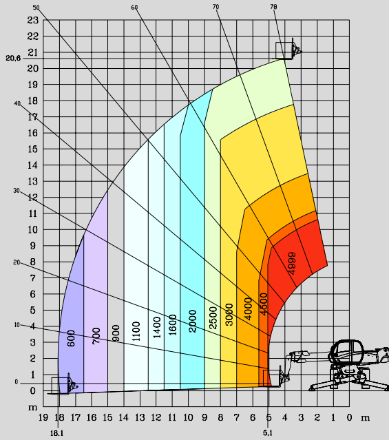
ROTATION ON STABILISERS FULLY EXTENDED WITH FORKS
